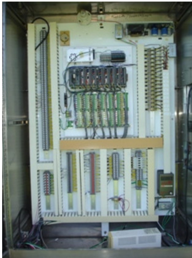
Fredericksburg RTU Cabinet Interior Elevation
