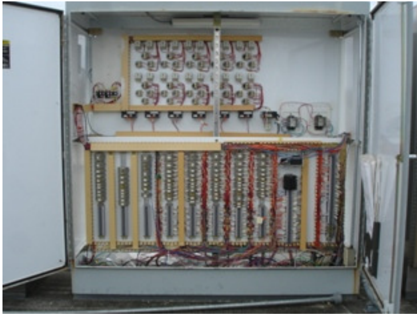
PSCP-03 Rear Interior Elevation
